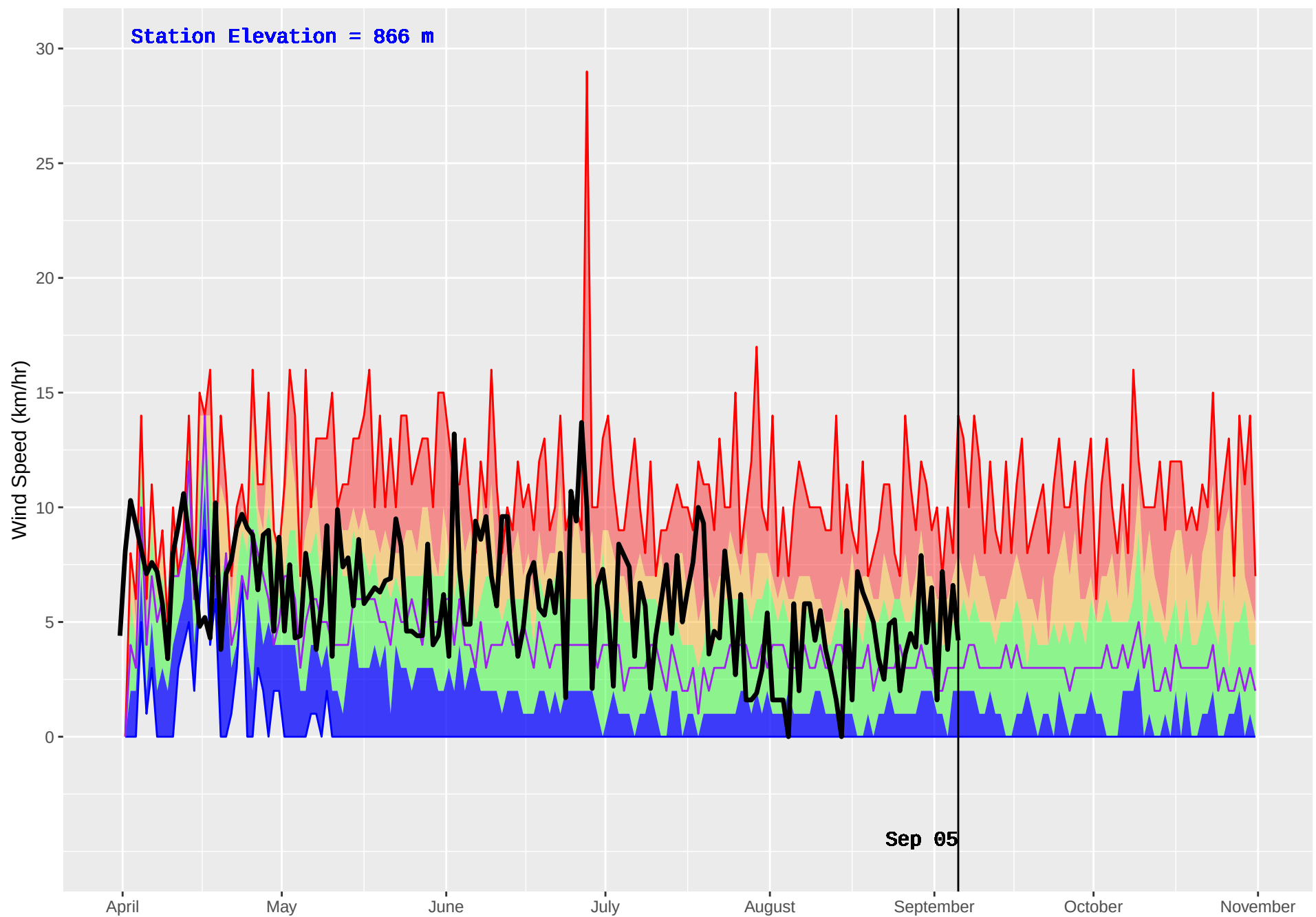
CATFISH (199) : Historical (1986–2016) and Current (2018) Daily Wind Speed
