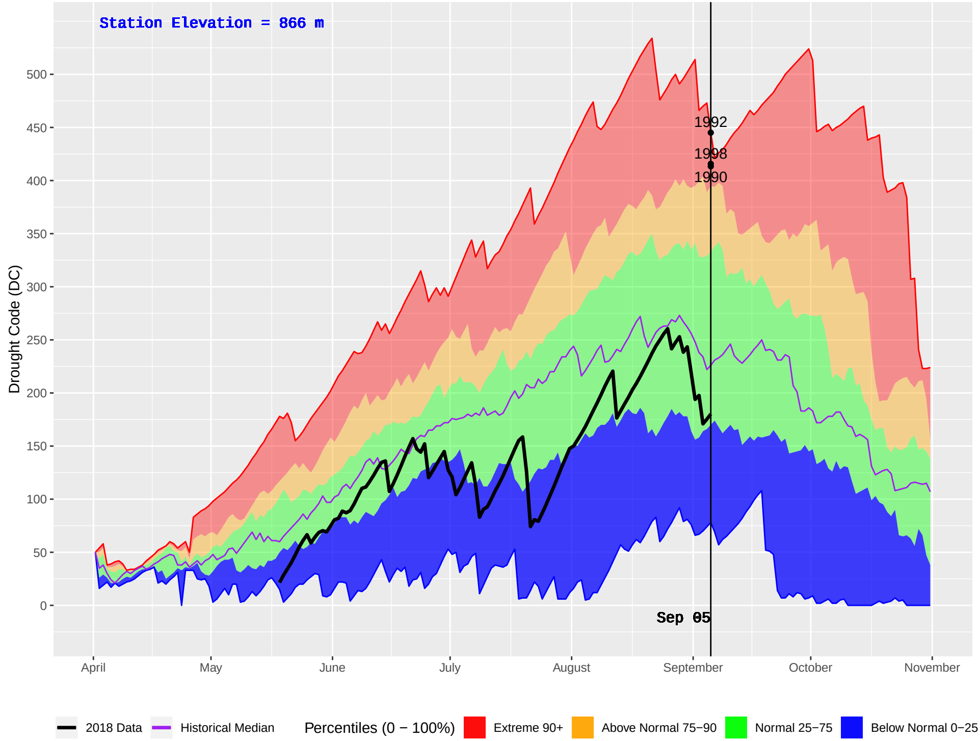
CATFISH (199) : Historical (1986–2016) and Current (2018) Daily Drought Code (DC)
